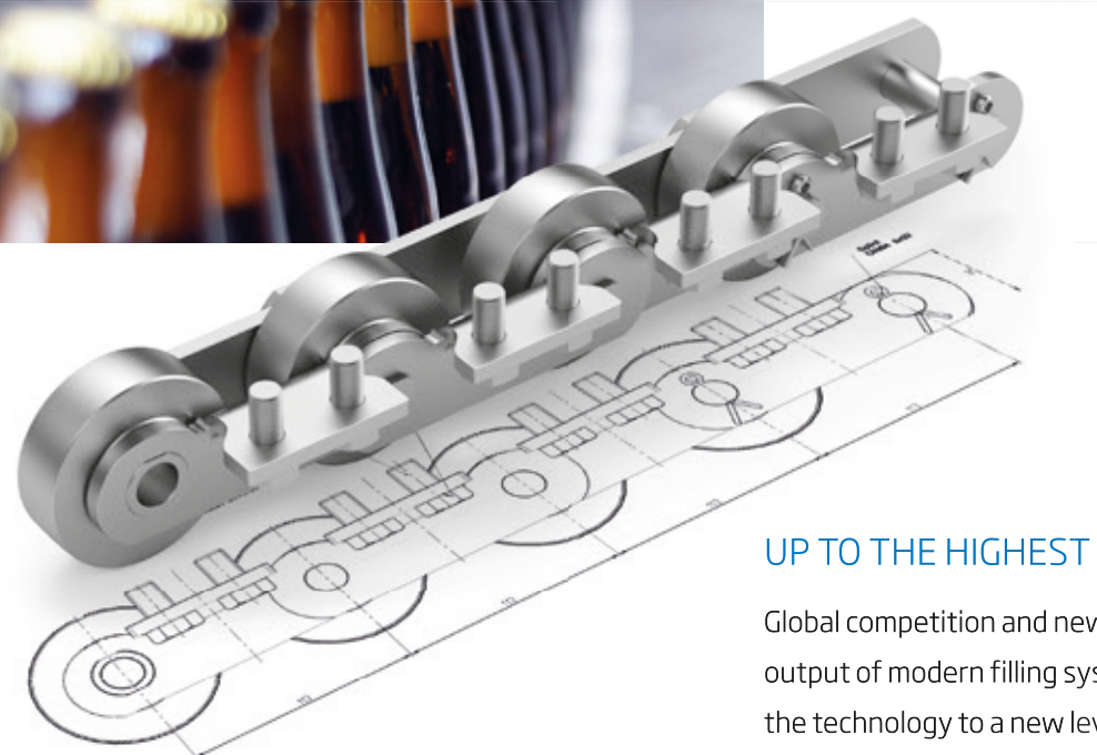
Chain for purification in the bottling industry with curved bracket
